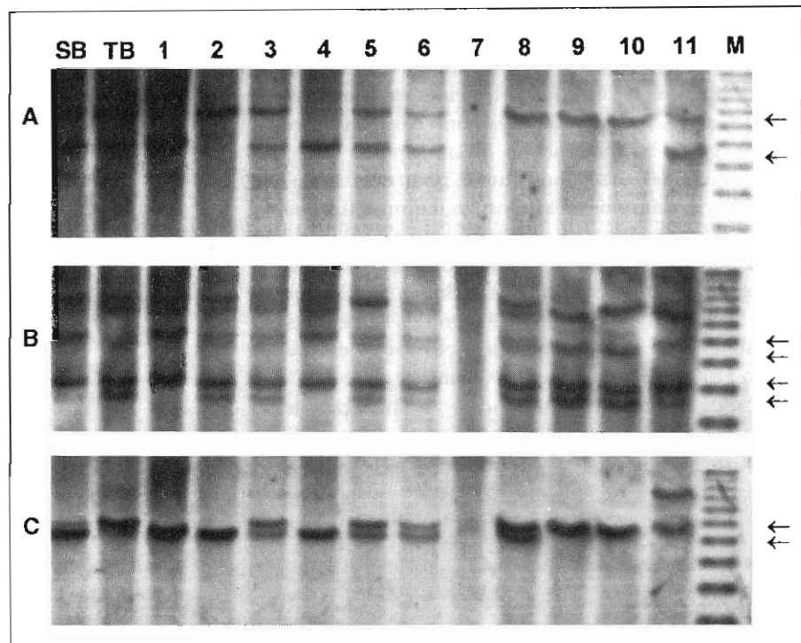
Figure 3 - Southern blots of bulked DNA samples and individual members of the bulks digested with EcoRI and probed with UMC103 (A), CSU155 (B) and UMC48 (C). SB, Al-susceptible bulk; TB, Al-tolerant bulk; 1 to 6, Al-susceptible individuals; 7 to 11, Al-tolerant individuals; M, molecular weight marker. Arrows indicate the polymorphic regions.
