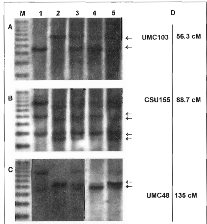
Figure 2 - Southern blots of parental and bulked DNA samples digested with EcoRI and probed with UMC103 (A), CSU155 (B) and UMC48 (C). Lane 1, L53 (Al-susceptible parent); lane 2, L1327 (Al-tolerant parent); lane 3, F 1 ; lane 4, Al-susceptible bulk; lane 5, Al-tolerant bulk; M, molecular weight marker. Arrows indicate the polymorphic regions. (D) Schematic representation of polymorphic markers location on chromosome 8 (Chao et al. , 1994).
